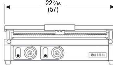
40795 Front and Side Views
