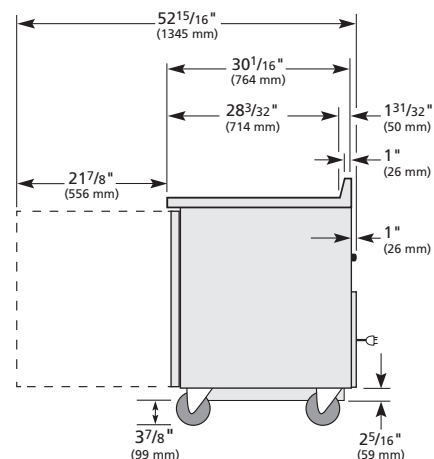
RIGHT VIEW
