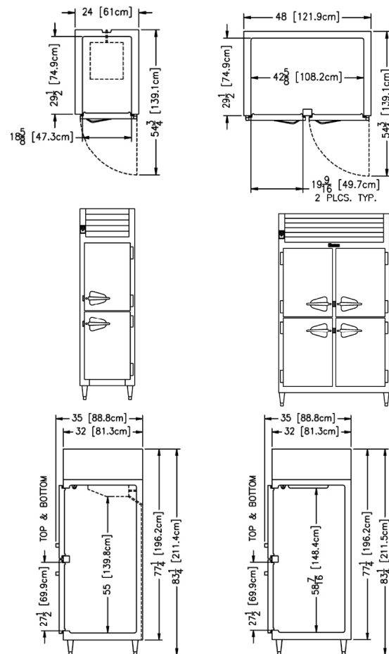
Section - R/ALT132DUT
